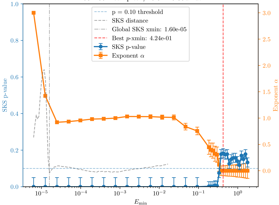
200x200 2 samples \gamma : 0.64 - 0.85umut
