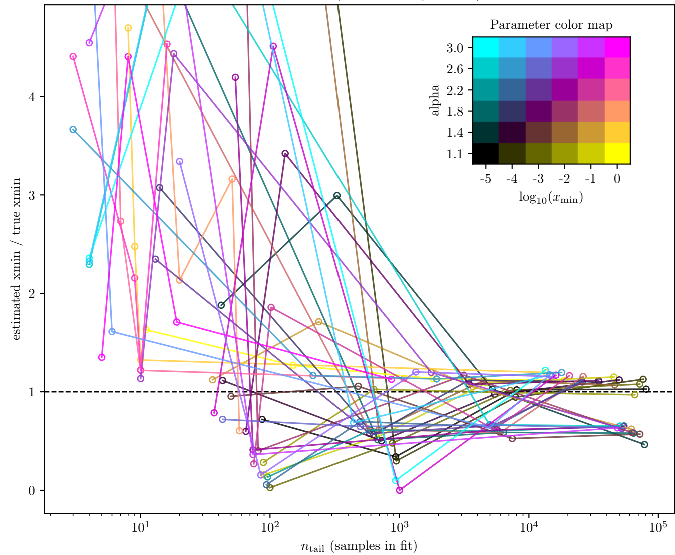
xmin estimate / true vs n (Plateau)
