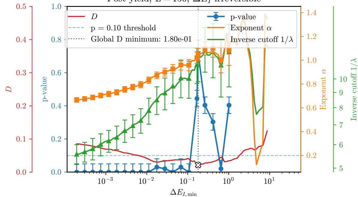
Post-yield, L = 150 ; \Delta E_I irreversible
