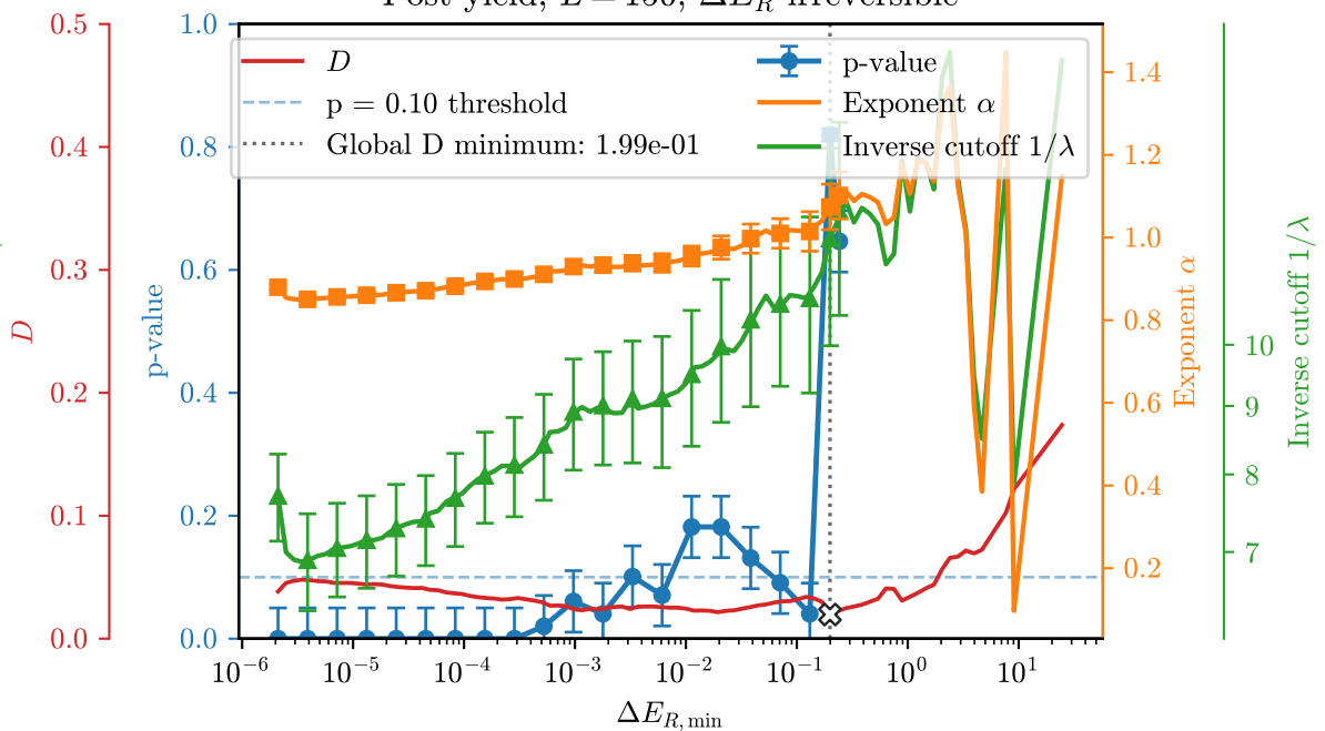
Post-yield, L = 150 ; \Delta E_R irreversible
