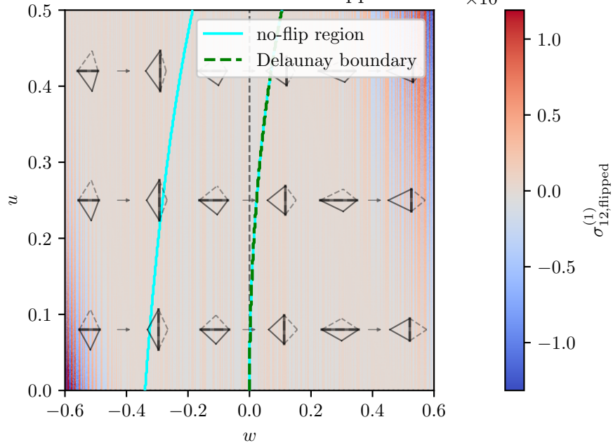
Element 1 shear stress flipped
