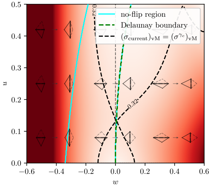
Element 1 von Mises stress current
