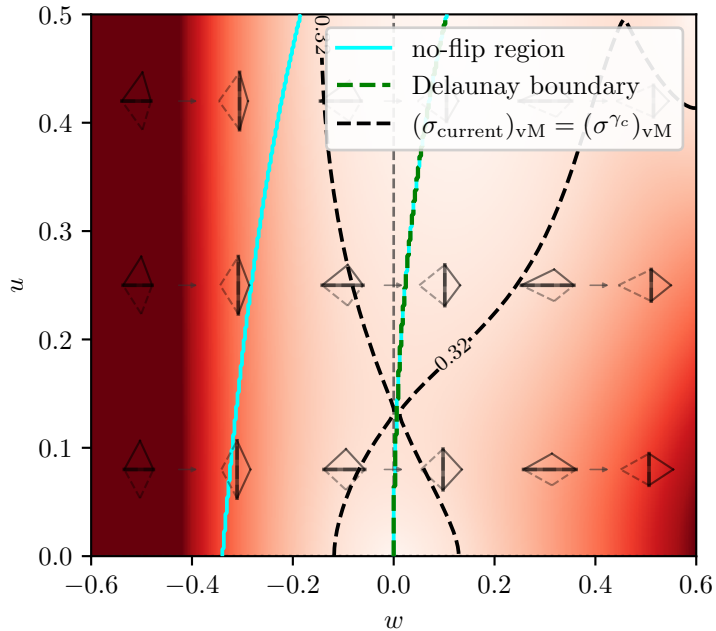
Element 2 von Mises stress current
