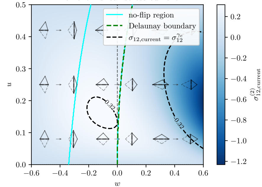
Element 2 shear stress current
