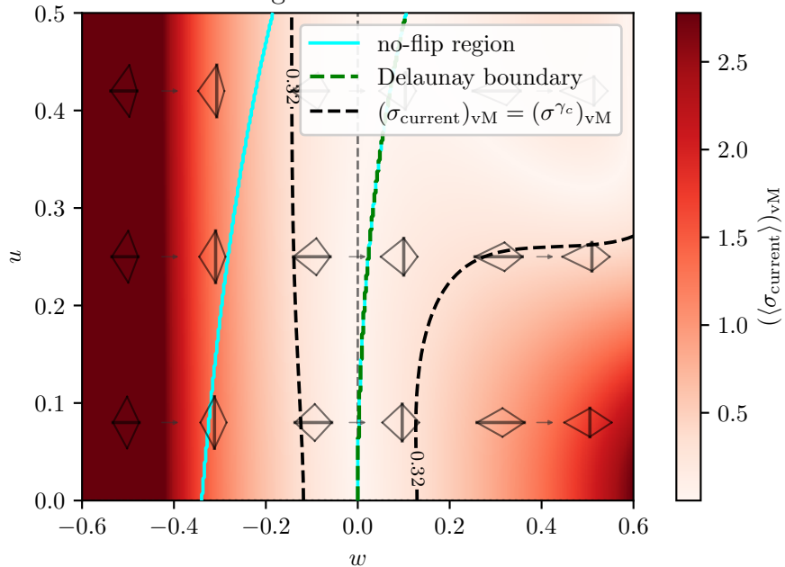
Element-averaged von Mises stress current
