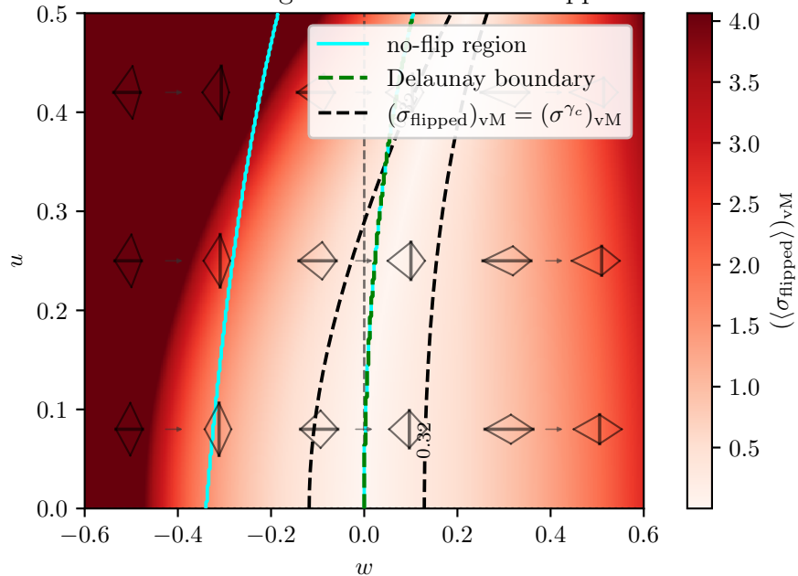
Element-averaged von Mises stress flipped
