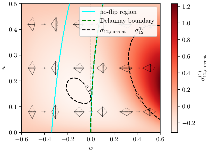
Element 1 shear stress current
