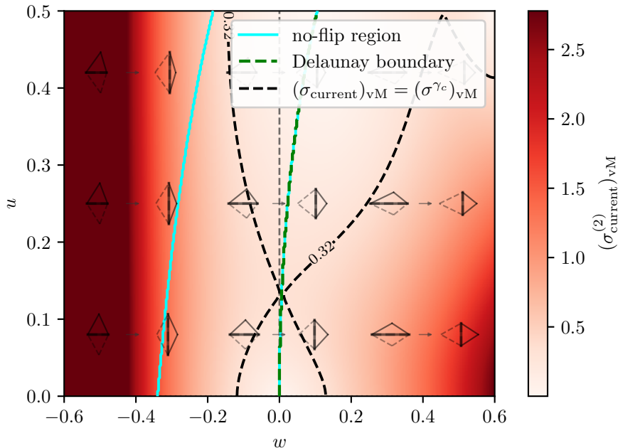
Element 2 von Mises stress current
