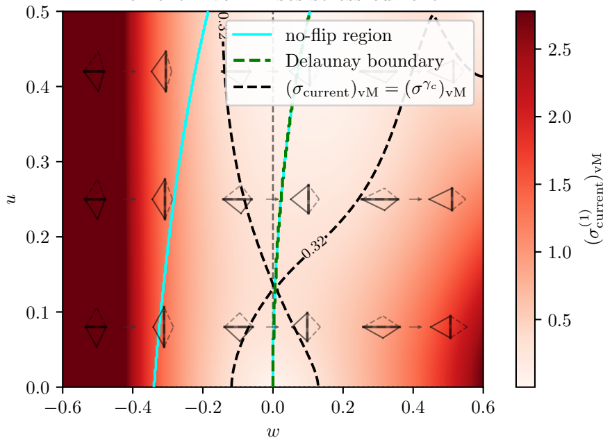
Element 1 von Mises stress current
