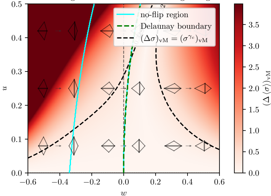
Element-averaged von Mises stress-change magnitude
