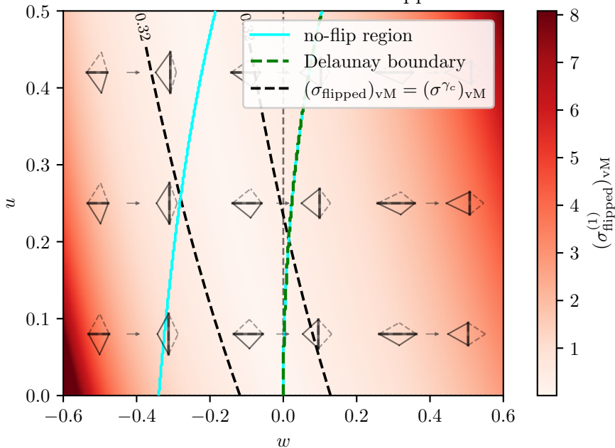
Element 1 von Mises stress flipped
