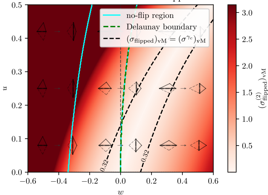
Element 2 von Mises stress flipped
