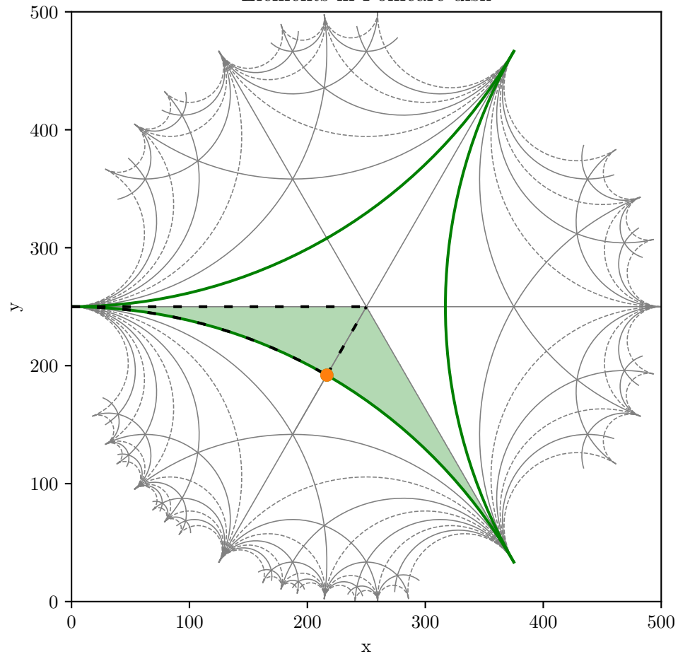
Elements in Poincaré disk
