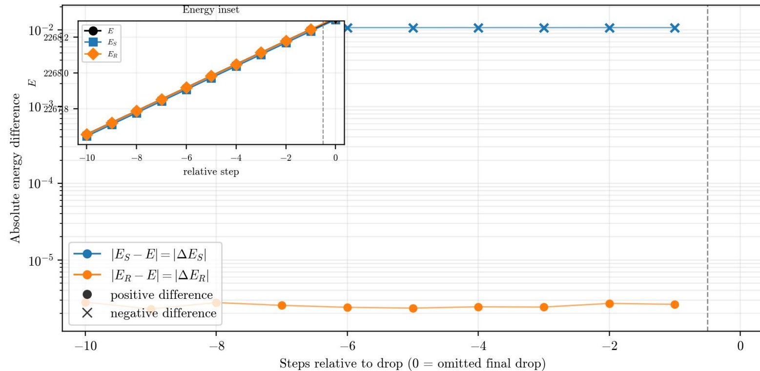
250x250 non-reconnecting energy-drop zoom irreversible sample 4/20, load=0.98356, yield load=0.53102 \Delta E_S=0.00107683 , \Delta E_R=0.0117569 shared \Delta E_S \in [0.000417, 0.0144] , \Delta E_{R, \text{det}}=3.91\text{e-}06
