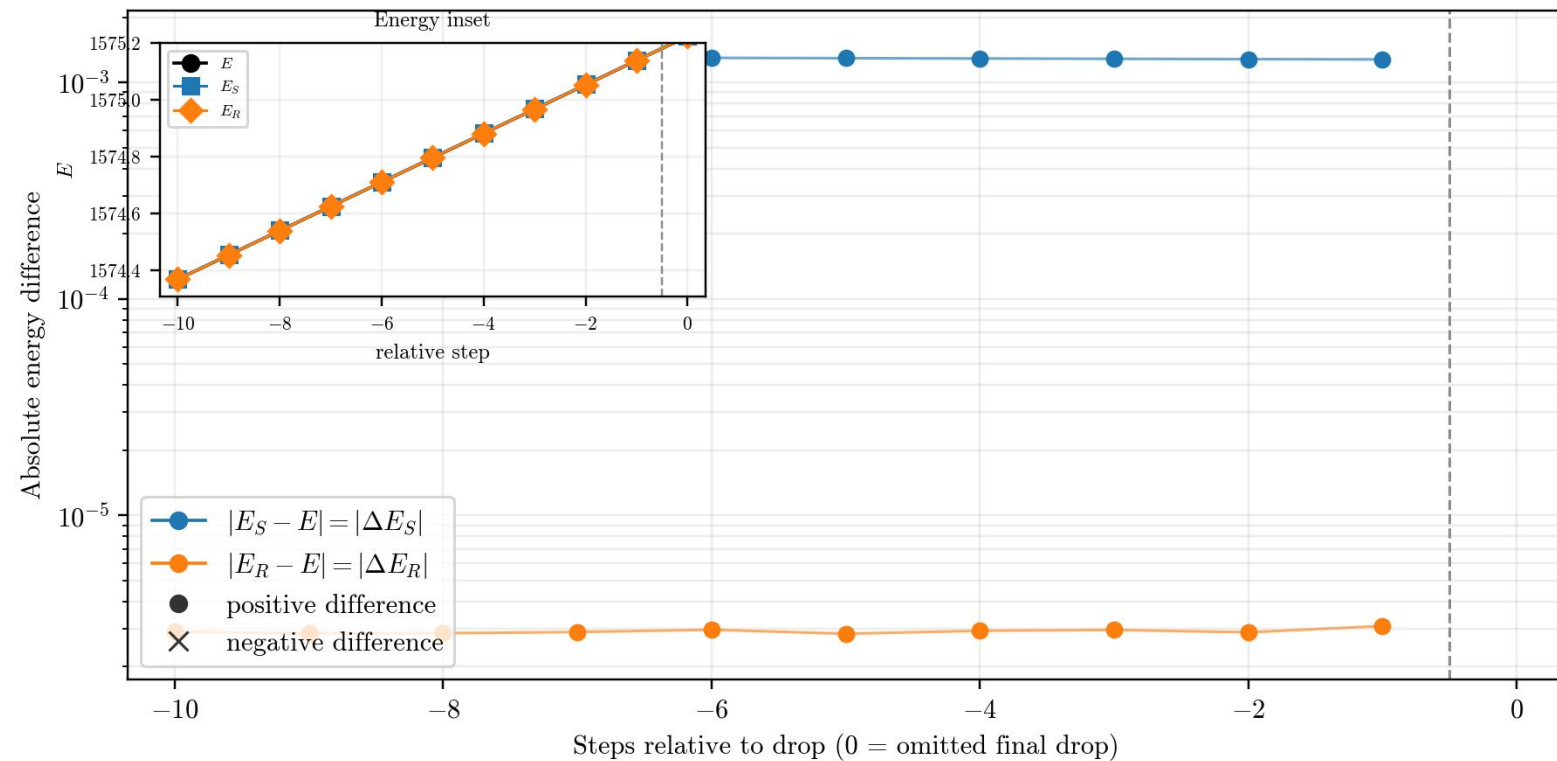
250x250 non-reconnecting energy-drop zoom irreversible sample 9/20, load=0.62283, yield load=0.53102 \Delta E_S=0.00184575 , \Delta E_R=0.000575308 shared \Delta E_S \in [0.000417, 0.0144] , \Delta E_{R, \text{det}}=3.91\text{e-}06
