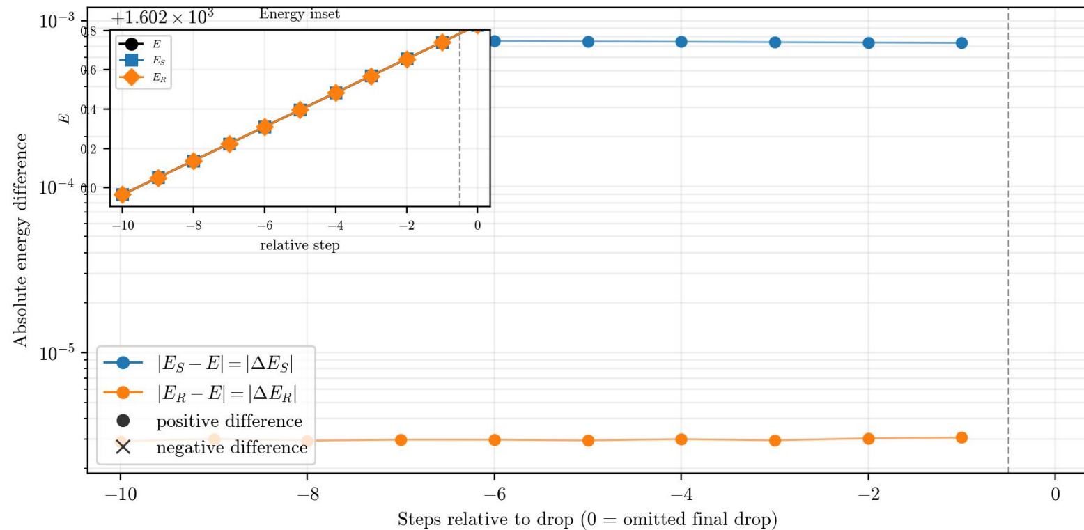
250x250 non-reconnecting energy-drop zoom reversible sample 4/20, load=0.63012, yield load=0.53102 \Delta E_S=0.000729173 , \Delta E_R=2.98451\text{e-}06 shared \Delta E_S \in [0.000417, 0.0144] , \Delta E_{R, \text{det}}=3.91\text{e-}06
