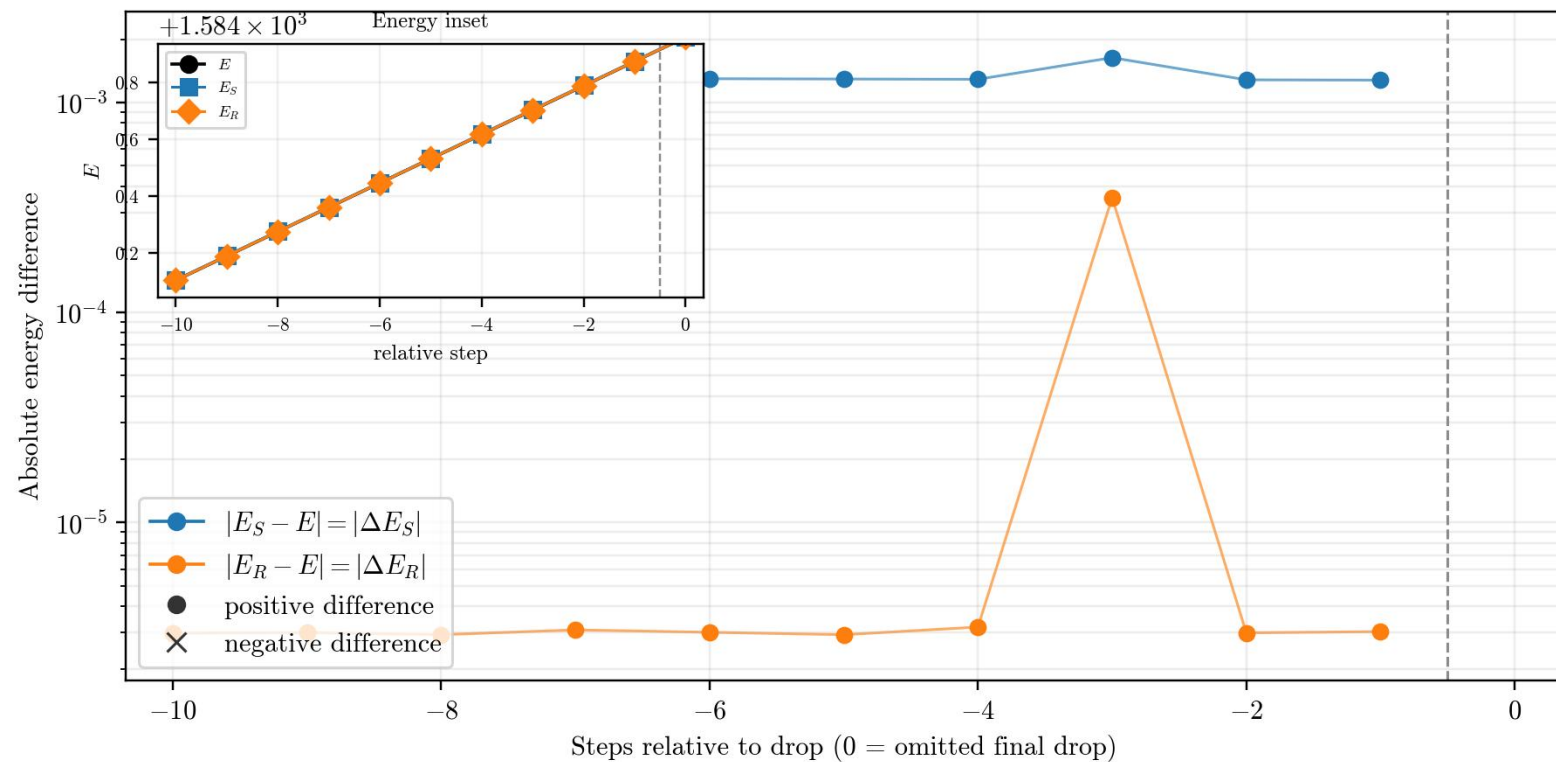
250x250 non-reconnecting energy-drop zoom reversible sample 7/20, load=0.62546, yield load=0.53102 \Delta E_S=0.00127501 , \Delta E_R=3.17005\text{e-}06 shared \Delta E_S \in [0.000417, 0.0144] , \Delta E_{R, \text{det}}=3.91\text{e-}06
