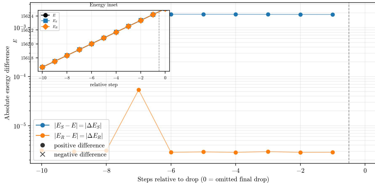
250x250 non-reconnecting energy-drop zoom reversible sample 9/20, load=0.62132, yield load=0.53102 \Delta E_S=0.00185012 , \Delta E_R=2.86148\text{e-}06 shared \Delta E_S \in [0.000417, 0.0144] , \Delta E_{R, \text{det}}=3.91\text{e-}06
