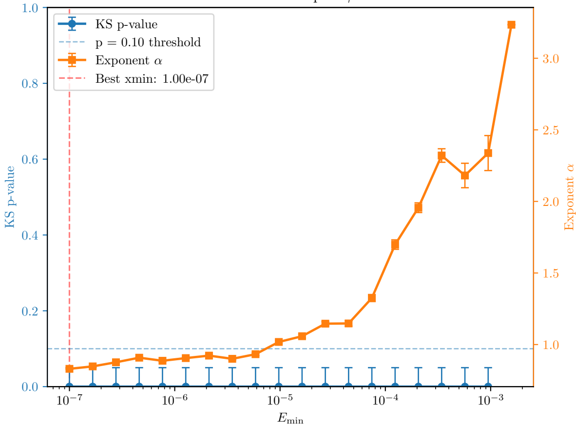
L-BFGS 100x100 40 samples \gamma : 0.15 - 1.00
