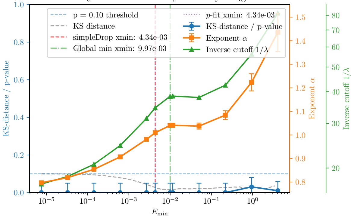
\Delta E_S irreversible events (selected by \Delta E_R )
