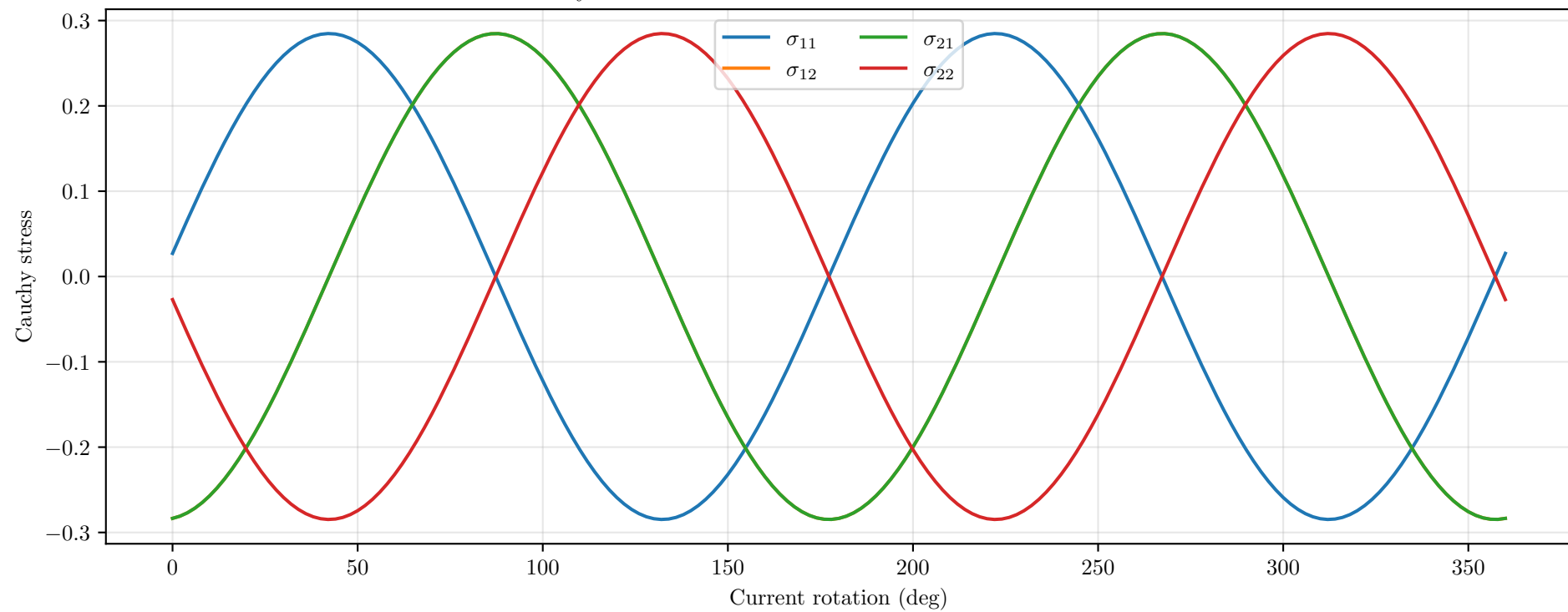
Cauchy stress for the same element under current rotation
