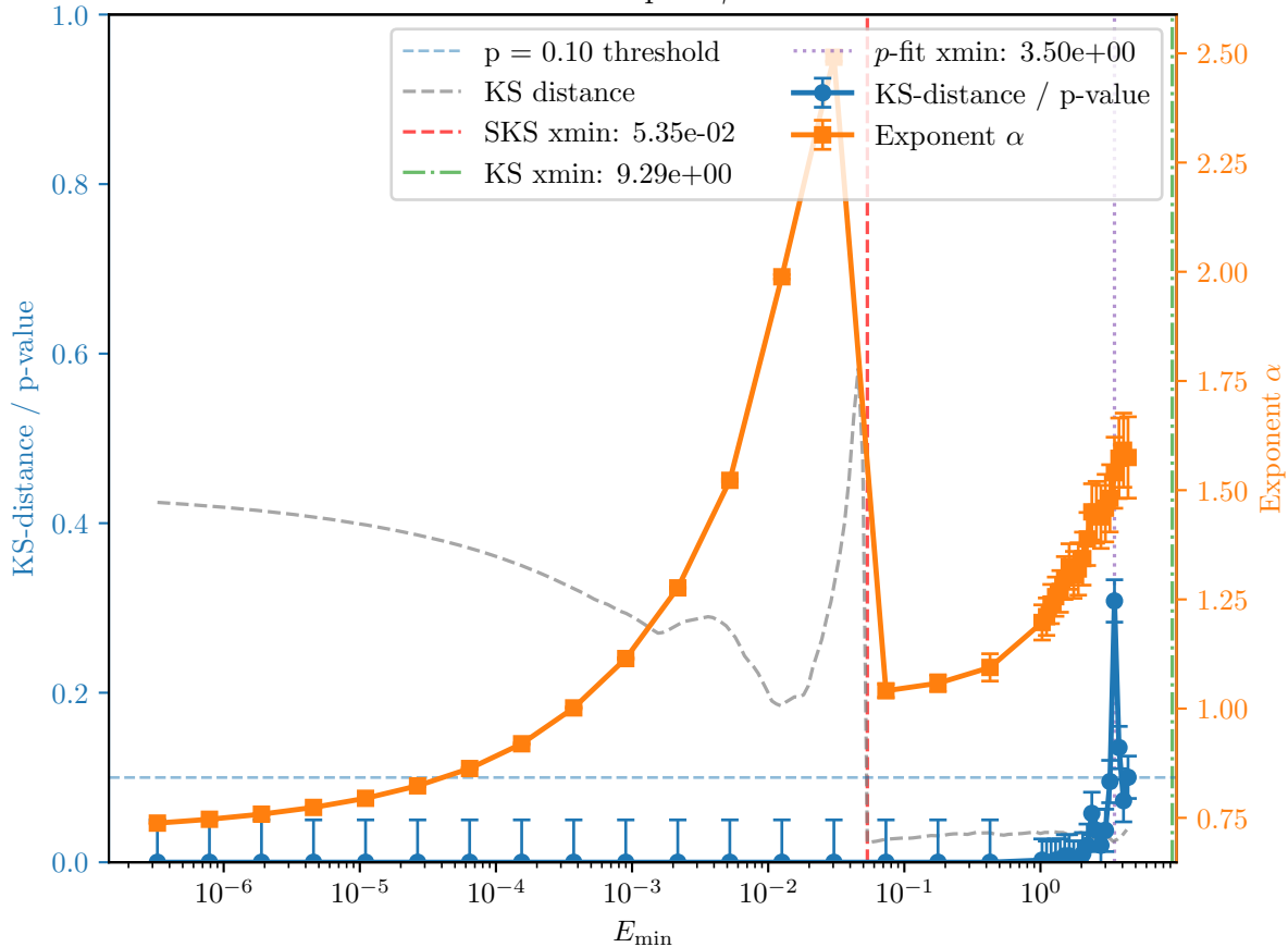
L-BFGS 200x200 10 samples \gamma : 0.57 - 0.97 L=200
