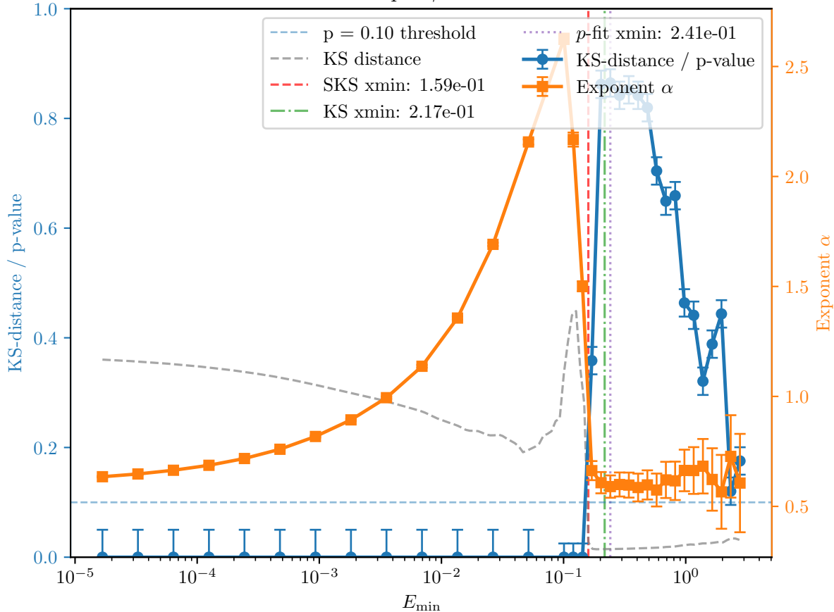
L-BFGS 500x500 1 sample \gamma : 0.14 - 0.53500x500Elias
