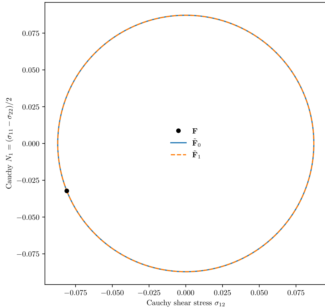
Rotated Cauchy-stress IDs
