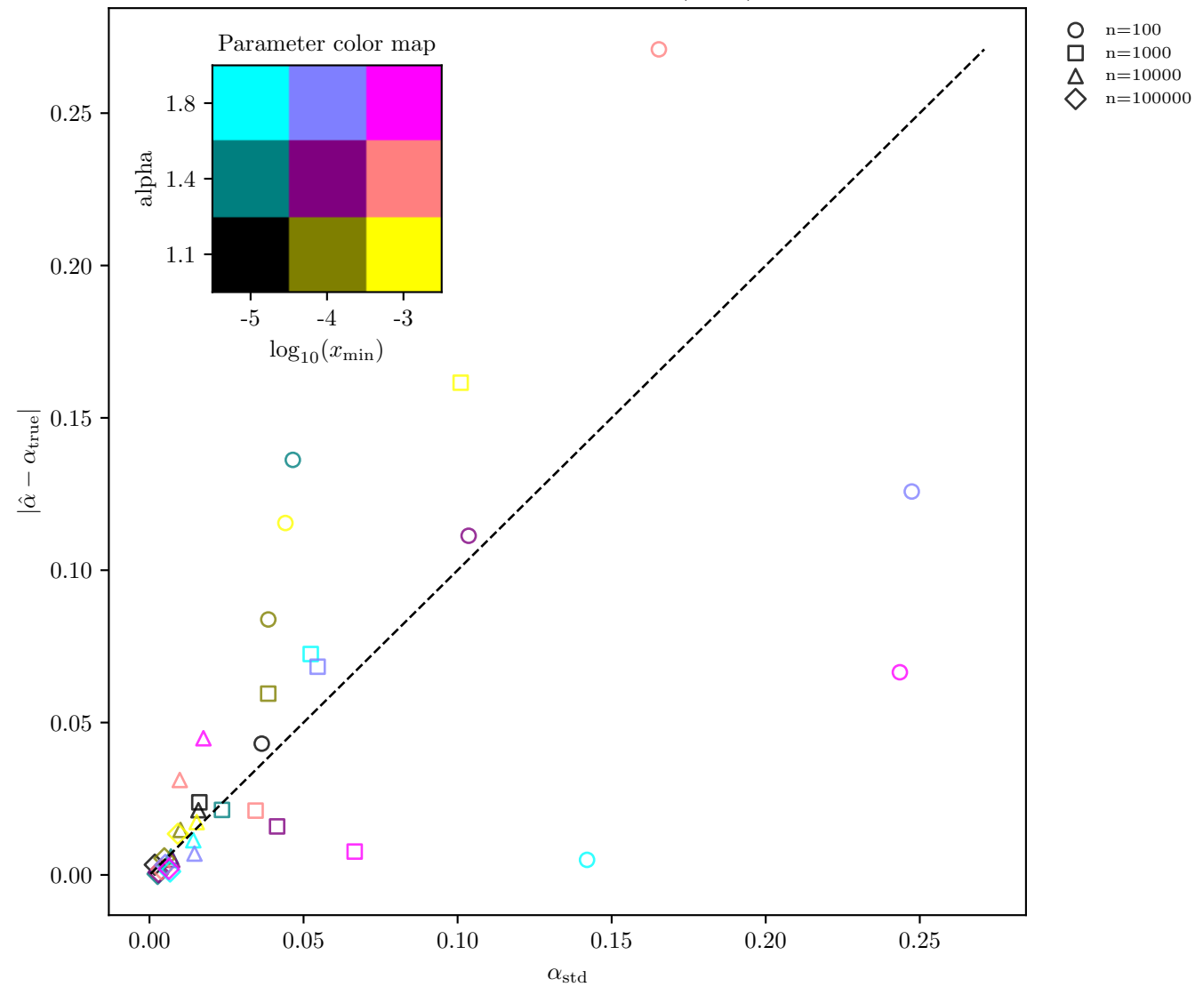
alpha error vs alpha std (DKS)
