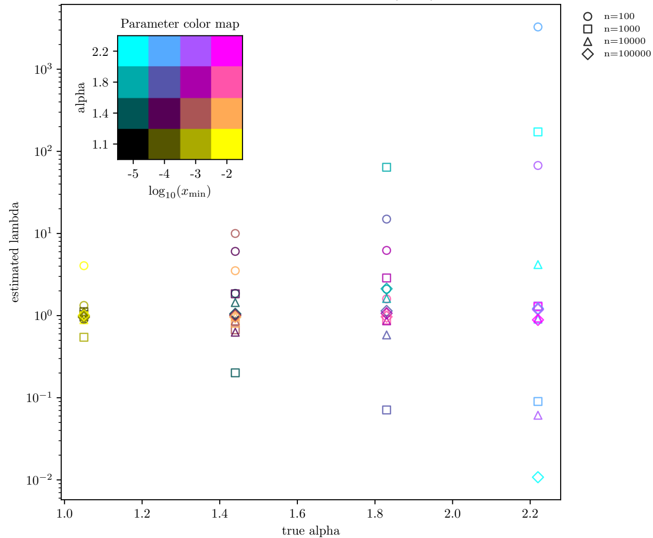
lambda estimate vs true alpha (DKS)
