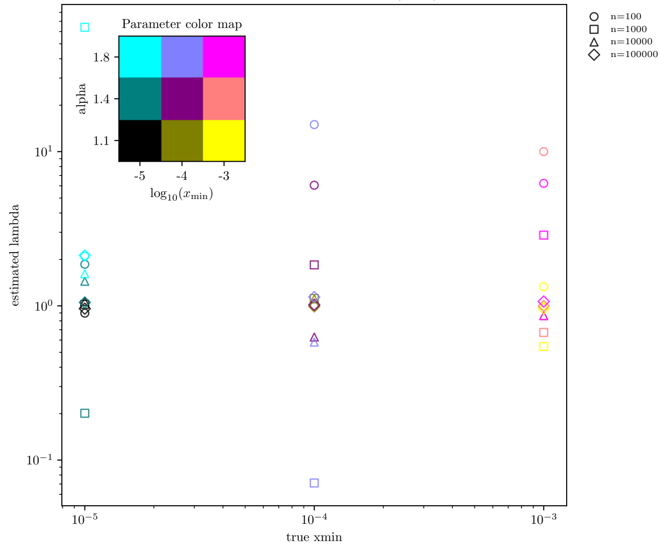
lambda estimate vs true xmin (DKS)
