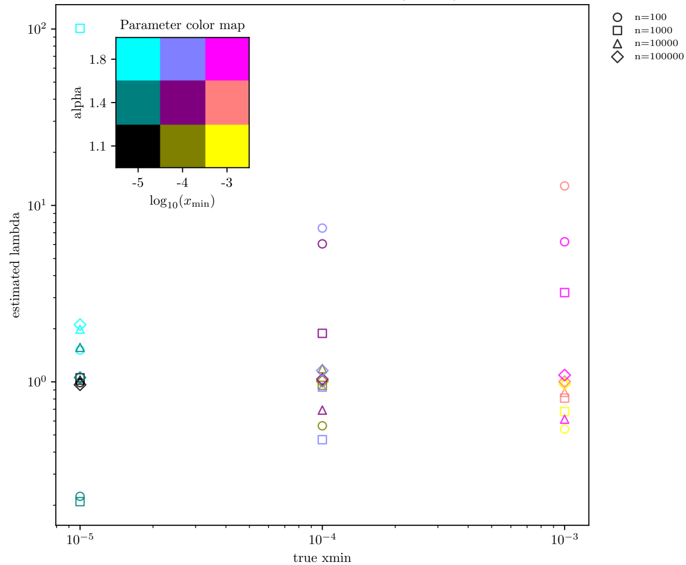
lambda estimate vs true xmin (minKS)
