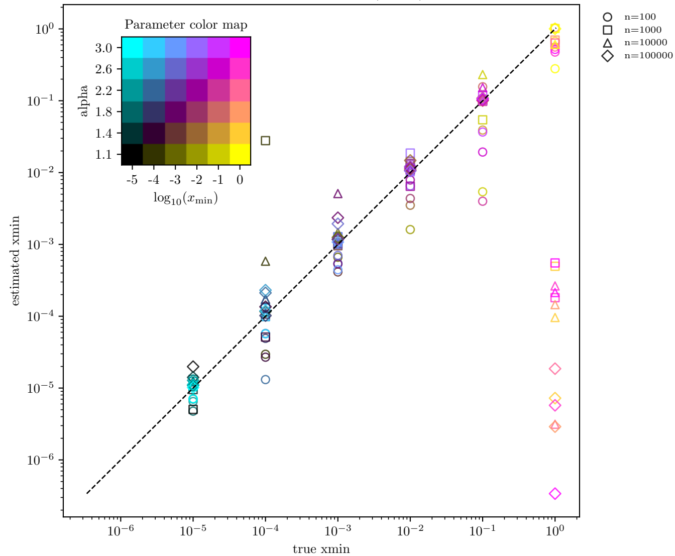
xmin estimate vs true (maxP)
