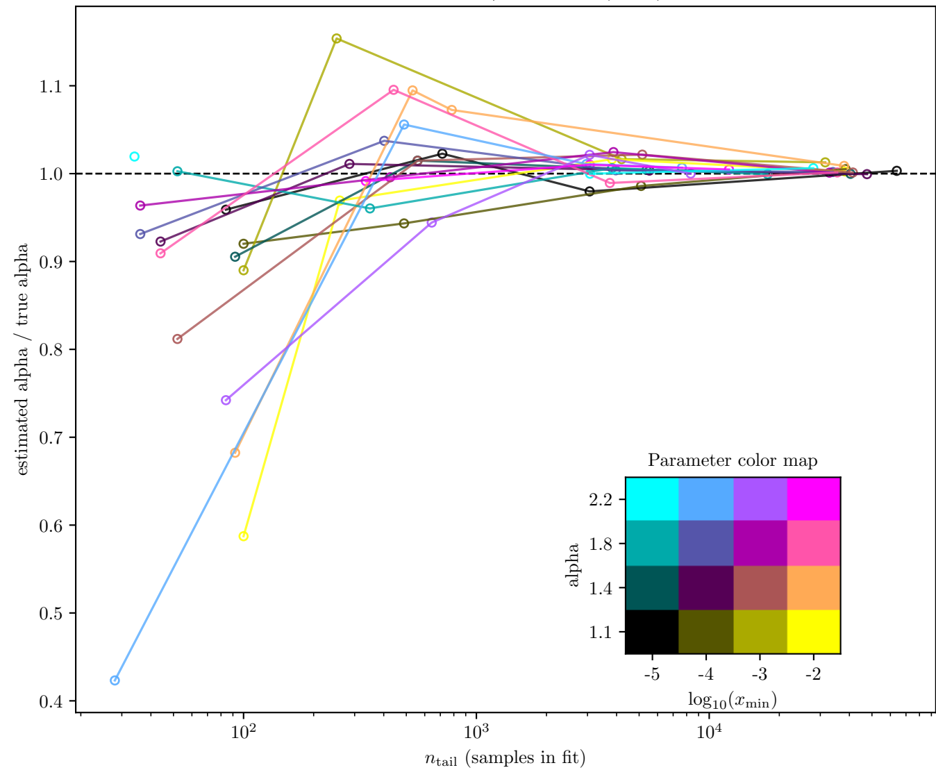
alpha estimate / true vs n (DKS)
