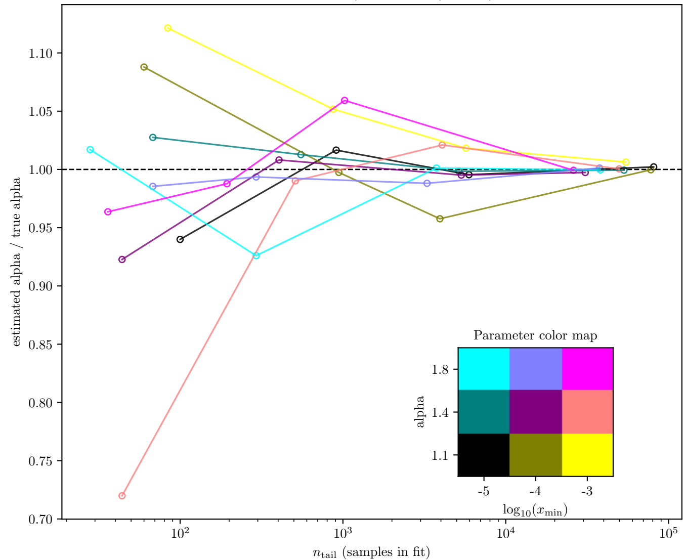
alpha estimate / true vs n (minKS)
