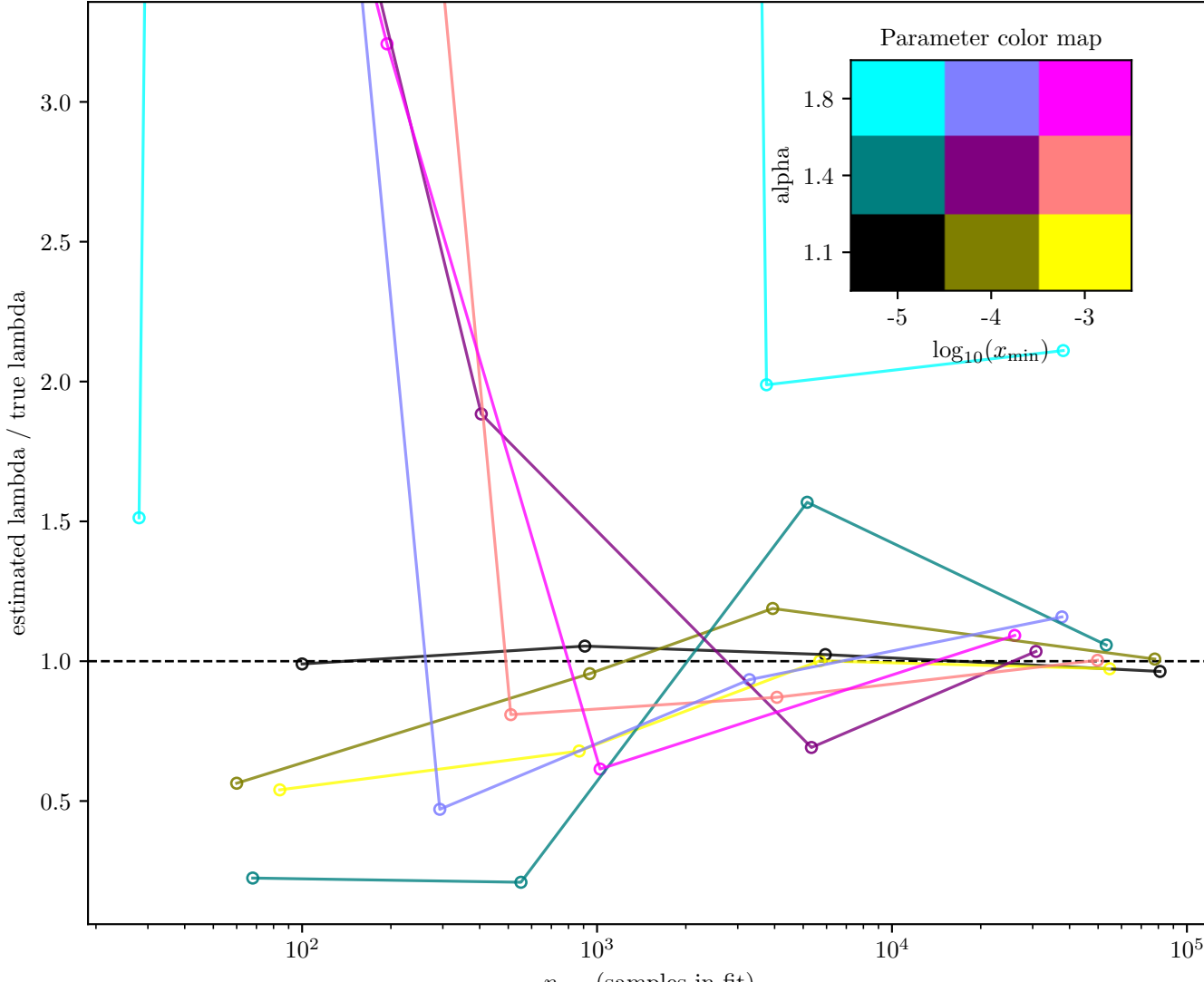
lambda estimate / true vs n (minKS)
