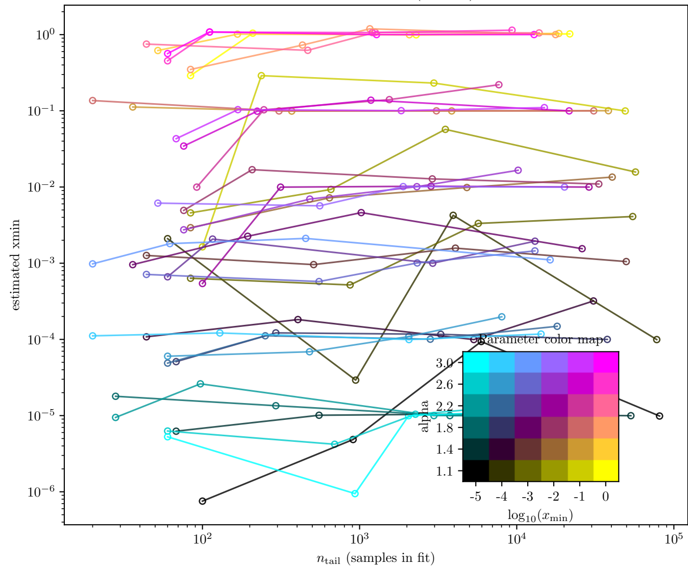
xmin estimate vs n (minKS)
