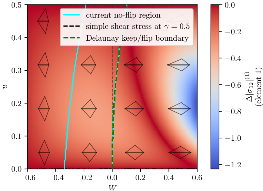
Element 1 absolute shear stress difference
