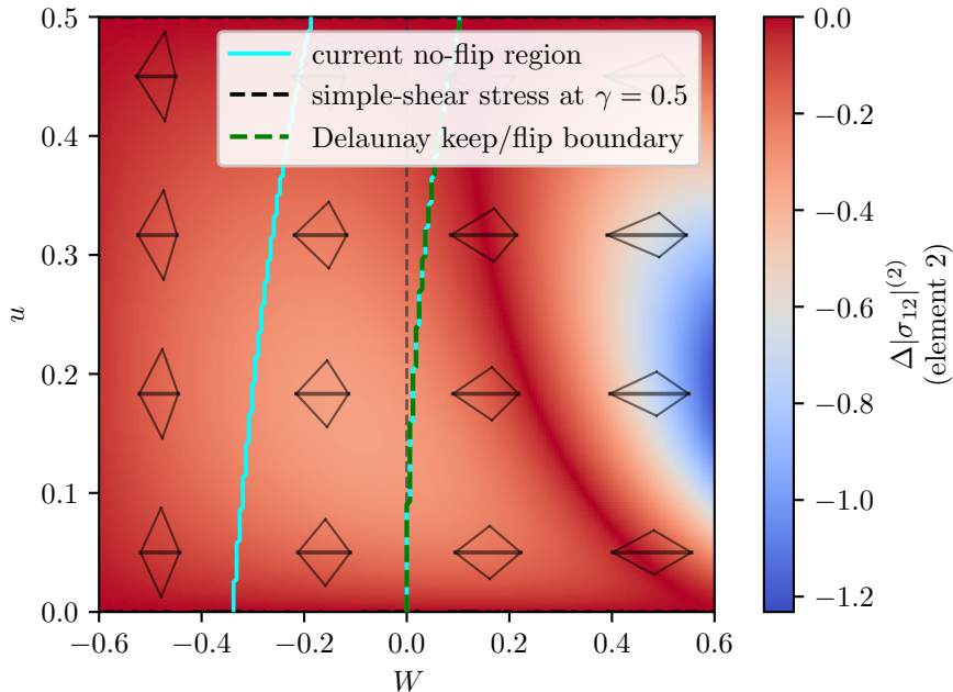
Element 2 absolute shear stress difference
