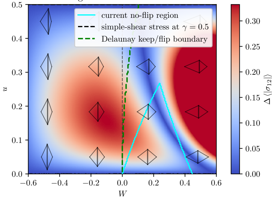
Element-averaged absolute shear stress difference
