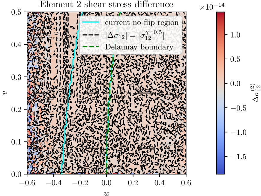
Element 2 shear stress difference
