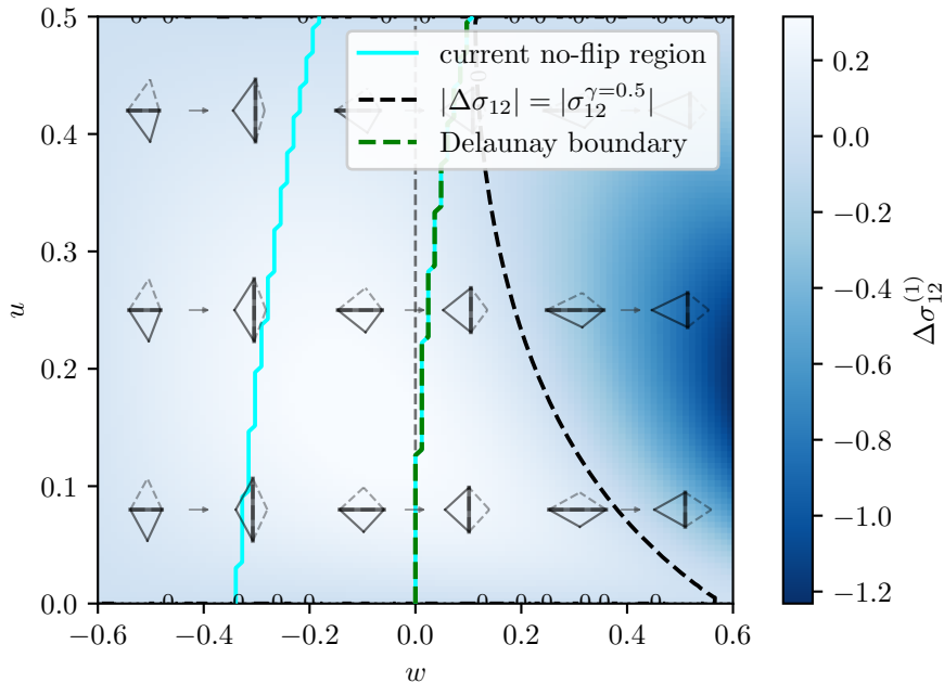
Element 1 shear stress difference
