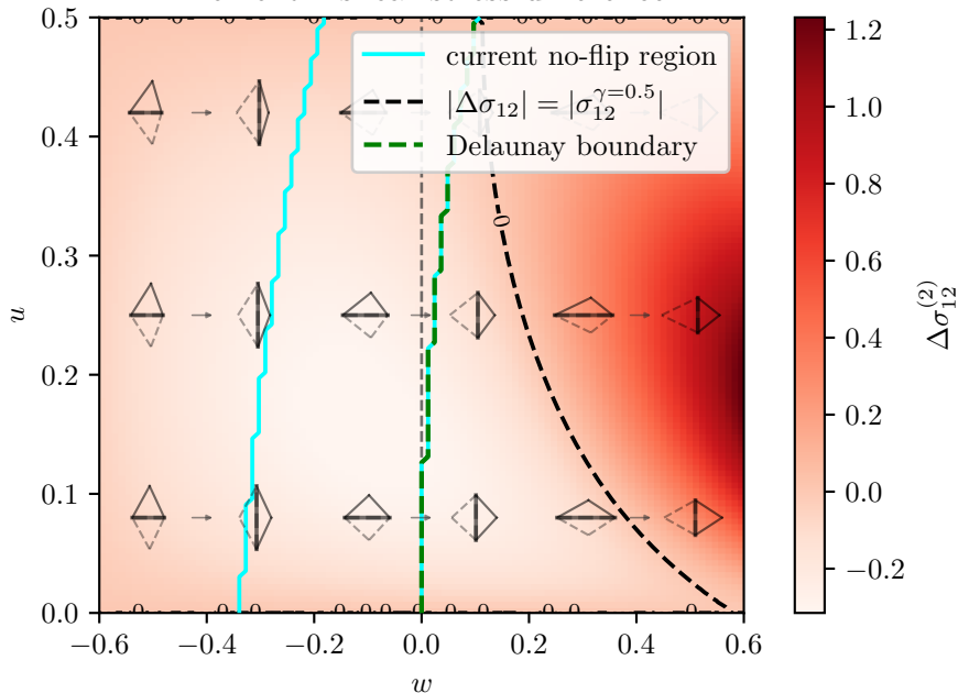
Element 2 shear stress difference
