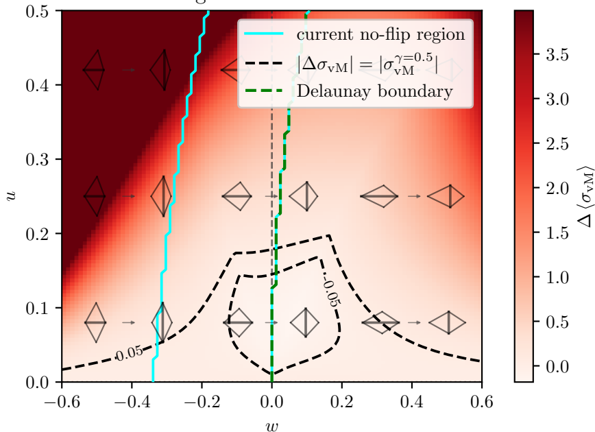
Element-averaged von Mises stress difference
