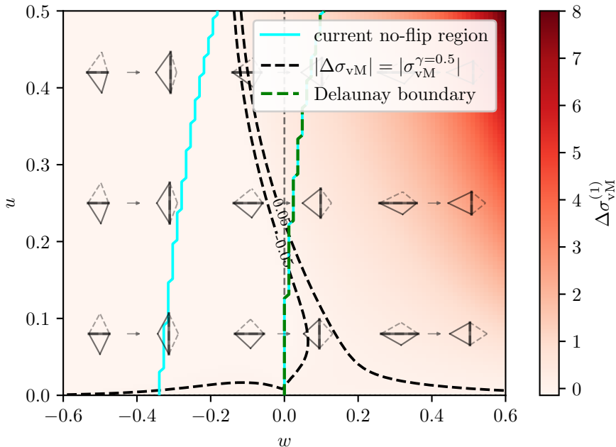
Element 1 von Mises stress difference
