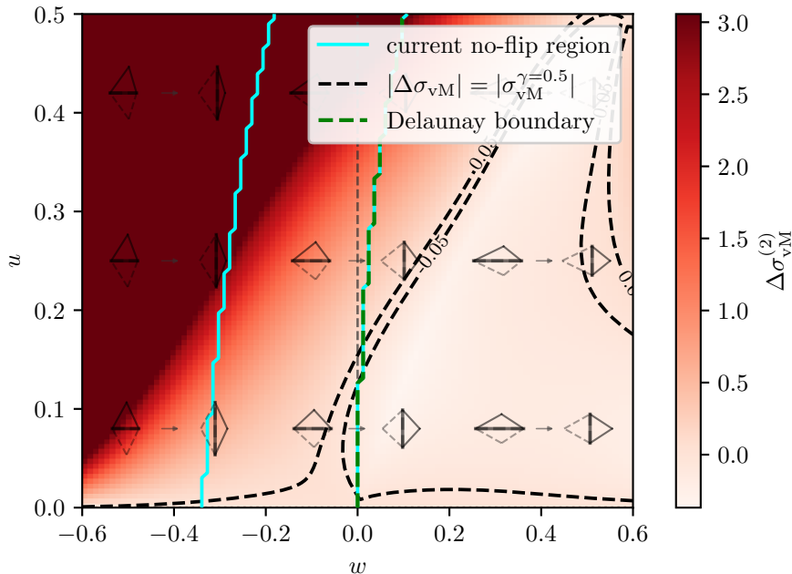
Element 2 von Mises stress difference
