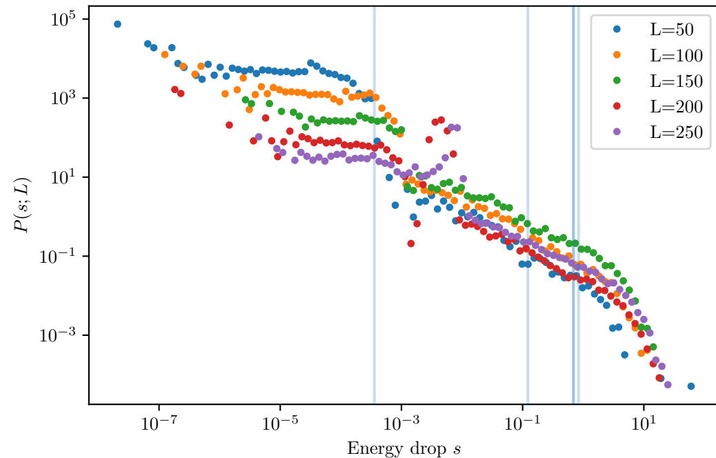
Second-order elastic continuation - pre-yield Per-size global_min xmin (vertical lines)
