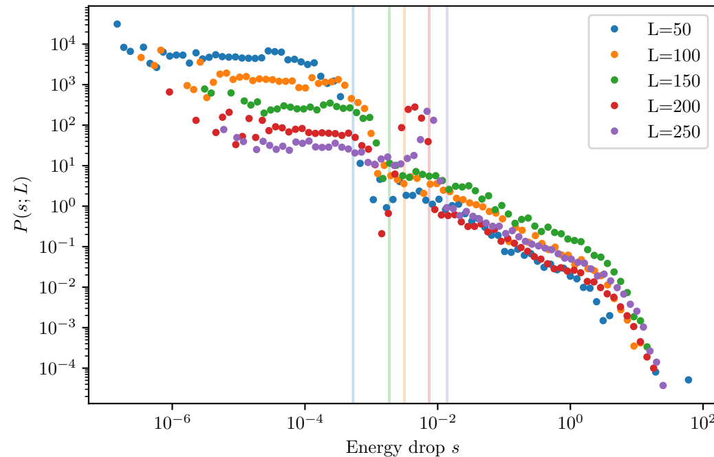
First-order elastic continuation - pre-yield Per-size plateau xmin (vertical lines)
