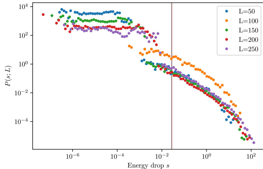
First-order elastic continuation - post-yield Shared xmin=2.758e-02 from L=250 (plateau)
