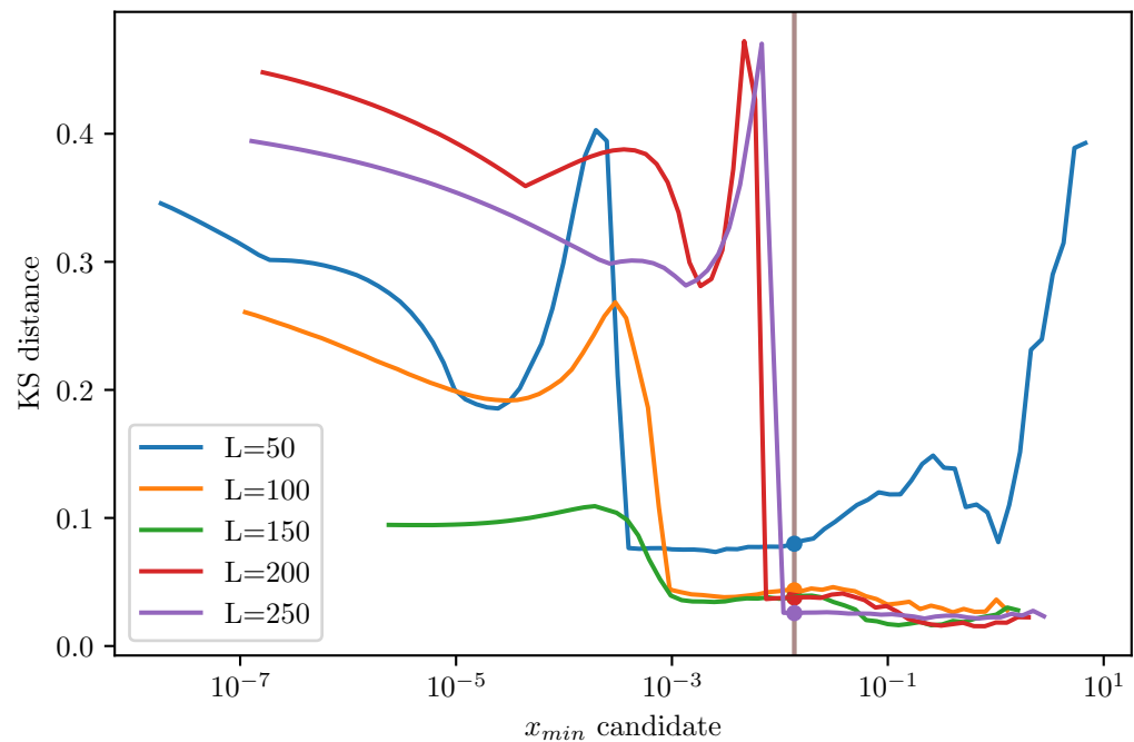
Second-order elastic continuation - pre-yield Shared xmin=1.361e-02 from L=250 (plateau)
