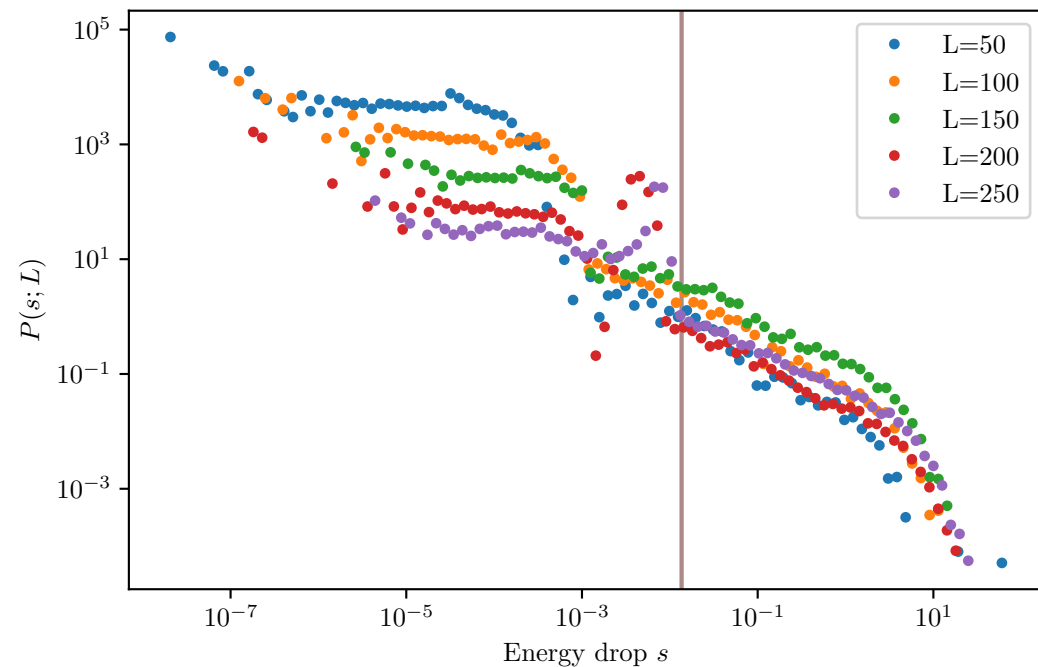
Second-order elastic continuation - pre-yield Shared xmin=1.361e-02 from L=250 (plateau)
