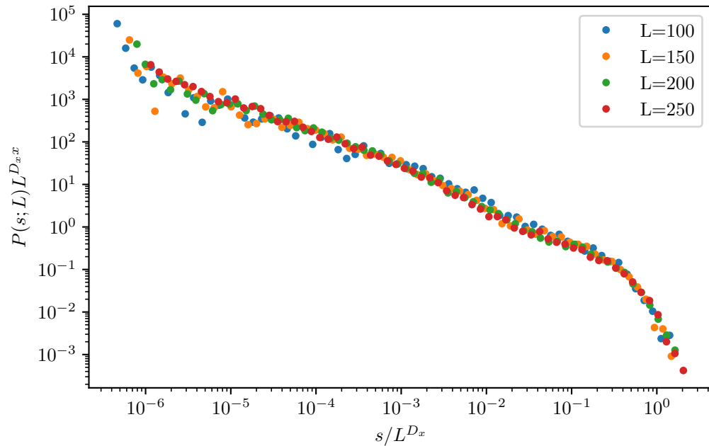
x = 0.500, D_x = 0.453
