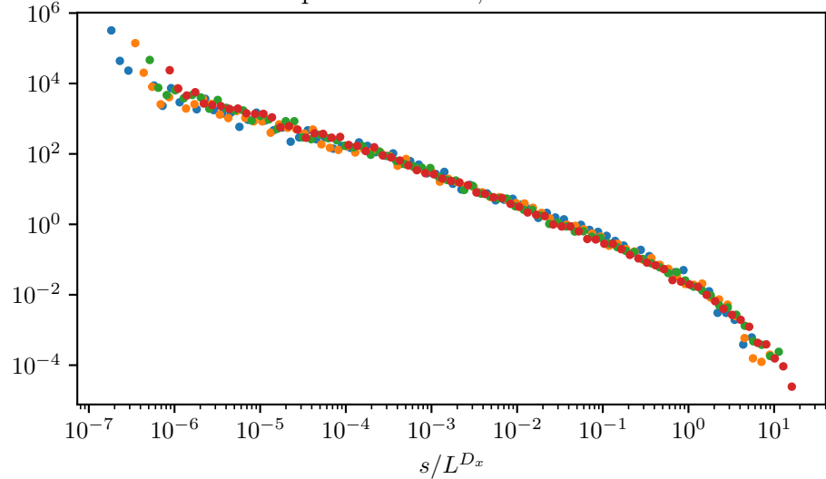
Affine initial-guess energy post: x=0.500 , D=0.382
