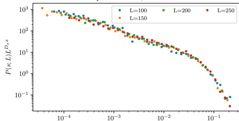
First-order elastic continuation pre: x=1.010 , D=0.887
