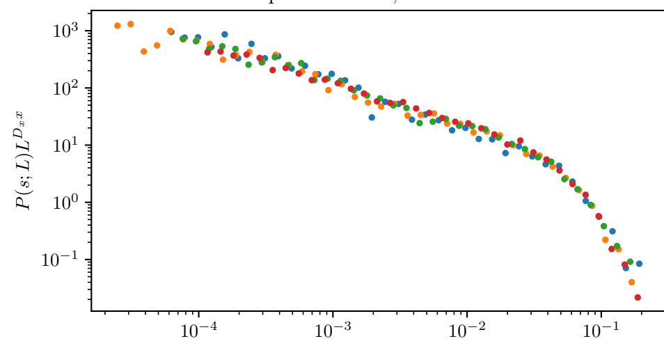
Previous relaxed energy pre: x=1.140 , D=0.868
