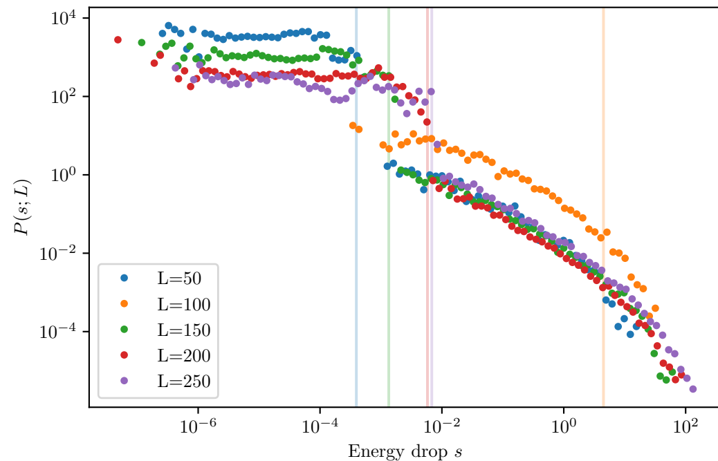
First-order elastic continuation - post-yield Per-size slope xmin (vertical lines)
