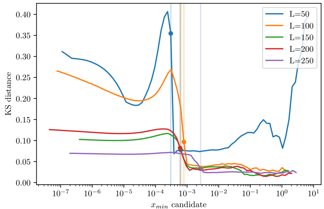
Previous relaxed energy - pre-yield Per-size slope xmin (vertical lines)
