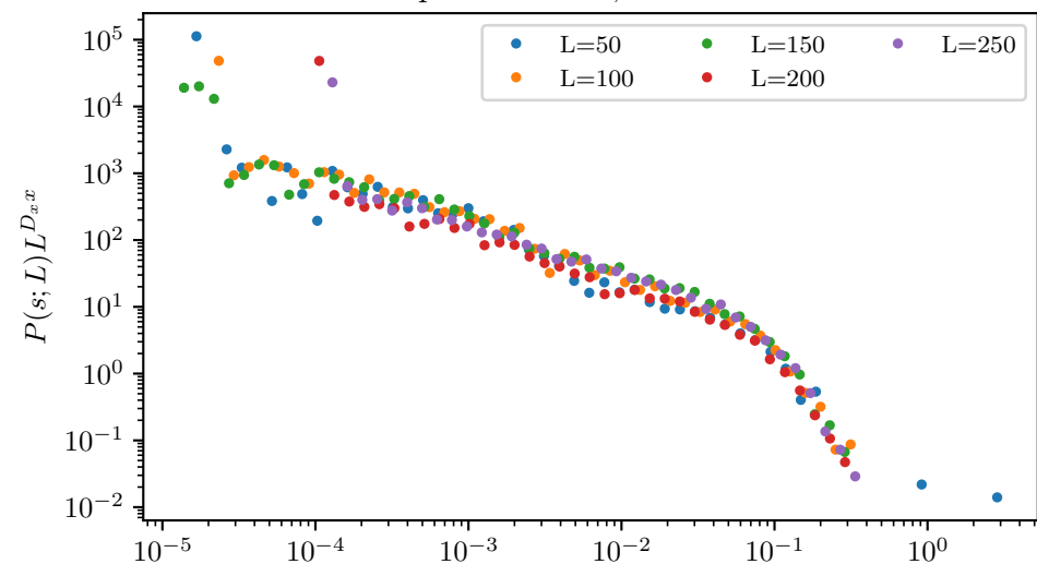
First-order elastic continuation pre: x=1.238 , D=0.772
