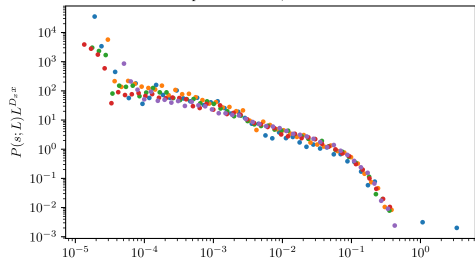
Affine initial-guess energy pre: x=0.500 , D=0.322
