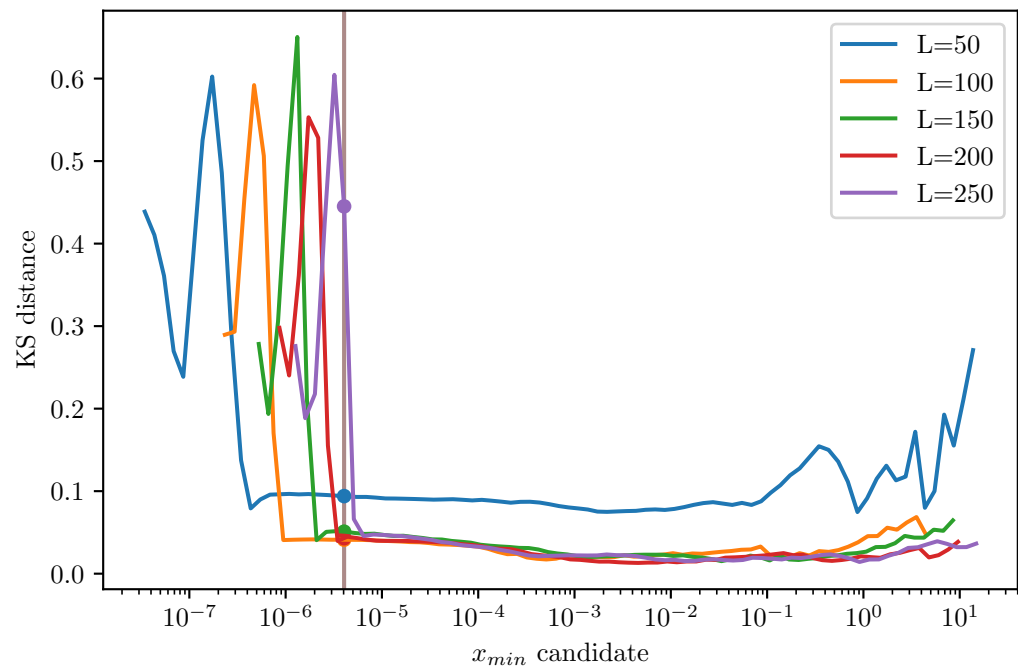
Affine initial-guess energy - post-yield Shared xmin=4.047e-06 from L=250 (slope)
