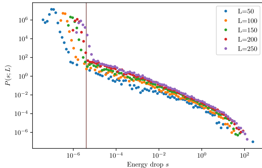
Affine initial-guess energy - post-yield Shared xmin=4.047e-06 from L=250 (slope)
