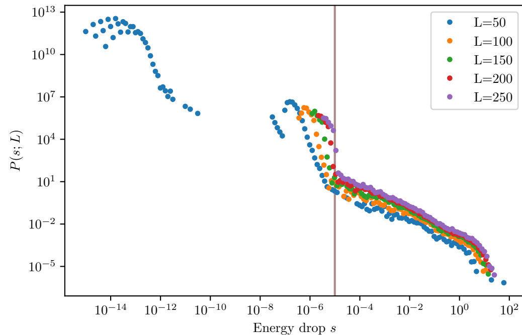
Affine initial-guess energy - pre-yield Shared xmin=9.918e-06 from L=250 (slope)
